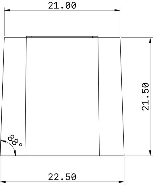
Back View
