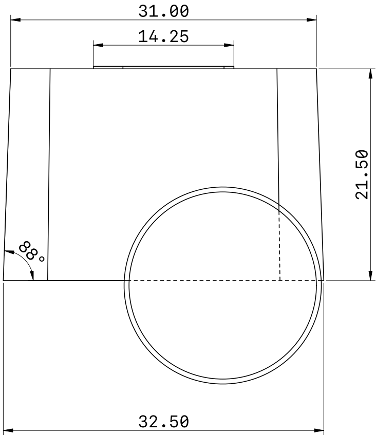
Right View
