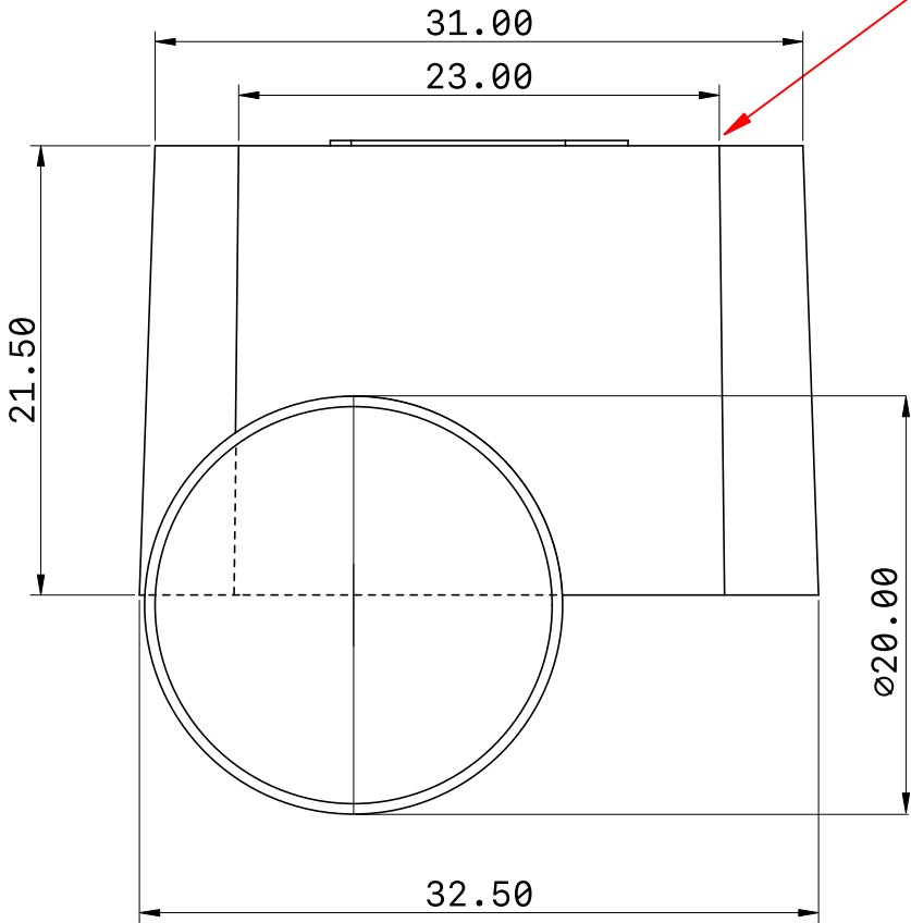
Left View
