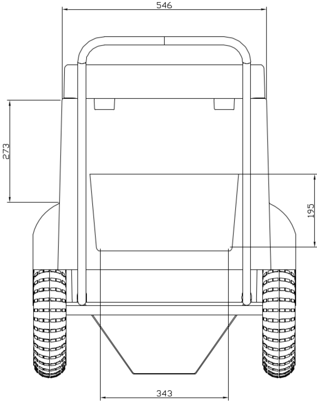
Rear
